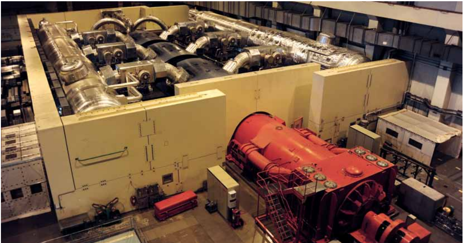
The high-pressure and low-pressure turbines are mounted along the same axis as the generator; the water separator/reheater can be seen to the left and right.
