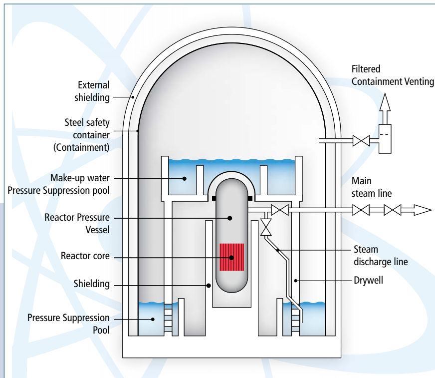
The cross-section of the Reactor Building shows the very solid structural barrier system. It protects the reactor from external influences while at the same time shielding the environment from radiation.
